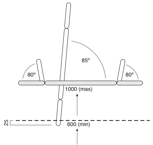
53821 Two Section
